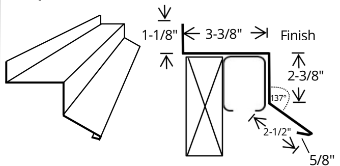
Square Track Cover
