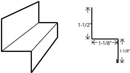
Inside Corner
