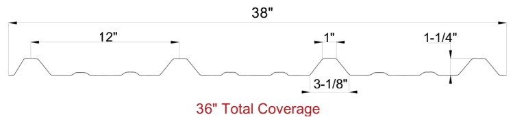
Pioneer Rib
