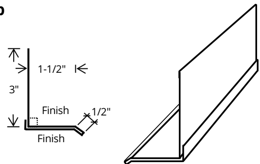
Com Drip Trim
