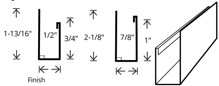
J Trim
