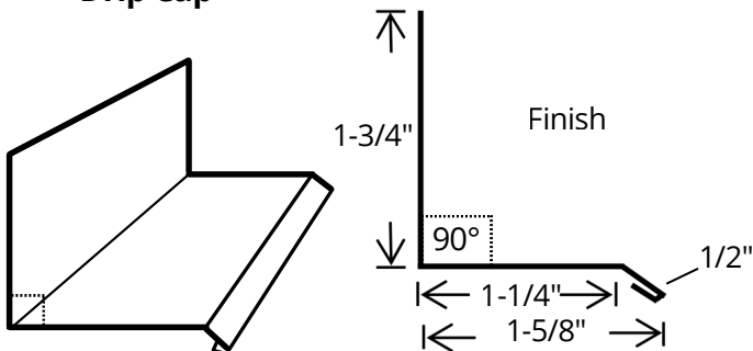
Drip Cap
