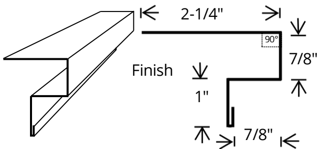
Drip Cap
