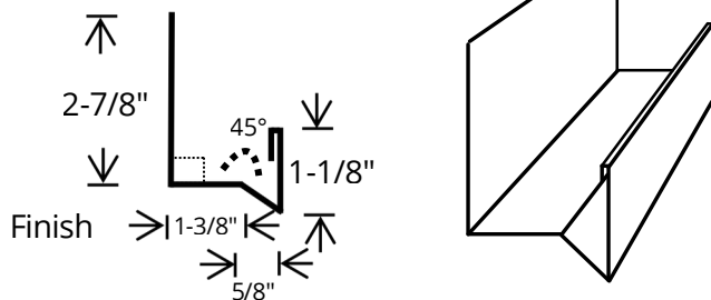
Com Header w/Drip
