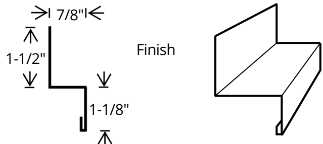
Transition - 7/8"
