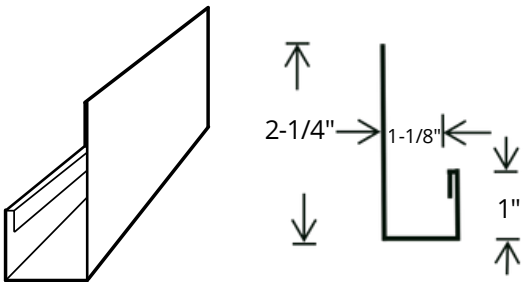
J-Channel
