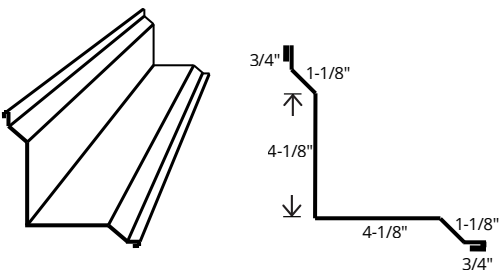
Inside Corner
