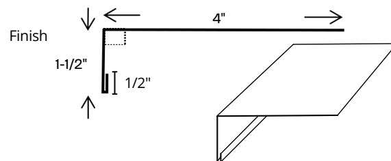
Com Window Sill Trim
