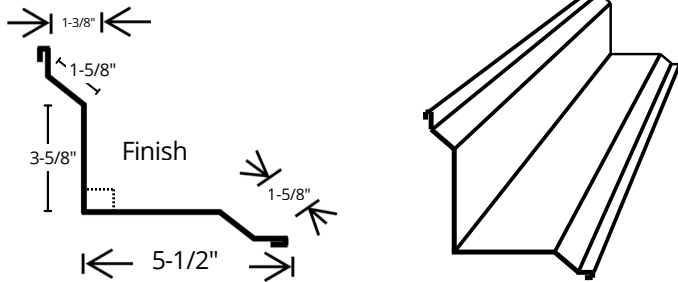
Com Inside Corner
