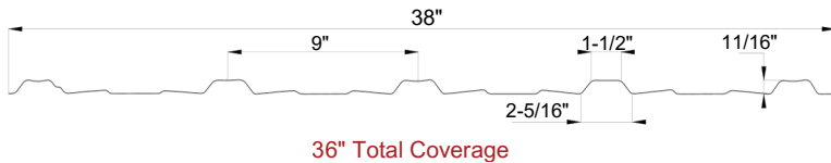
Continuous Rib Panel
