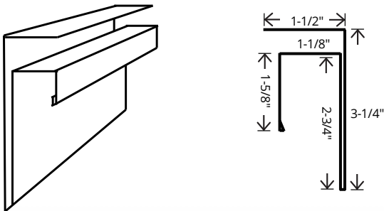
Soffit Starter
